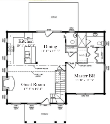
1st FLOOR PLAN (1,024 S.F.)
